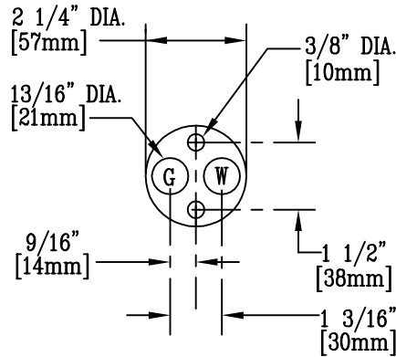
GUIDE WASHER DETAIL
